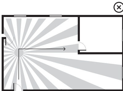
Figure 4: The sensor takes longer to detect movement when fewer zones are crossed.
