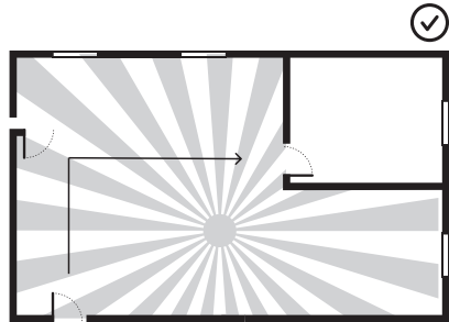
Figure 2: For faster detection, place the sensor away from the pathways between the doors.
